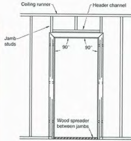
Figure 12 – Steel stud wall construction
